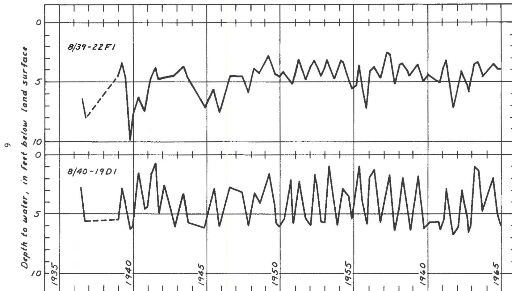
Figure 4.--Hydrographs of two wells in Baker Valley for the period 1936-64.
