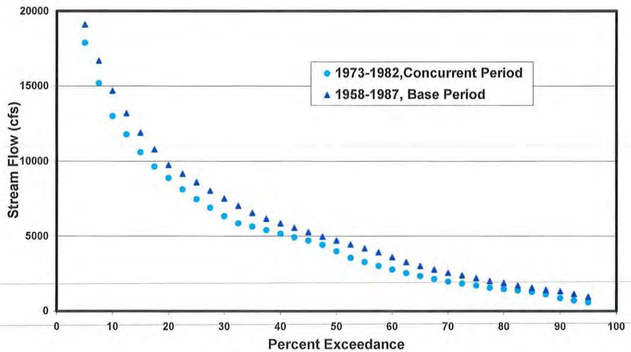
Figure 8. January Concurrent and Base Period Flow Duration Curves for the Nehalem River near Foss, OR - Gage 14301000.
