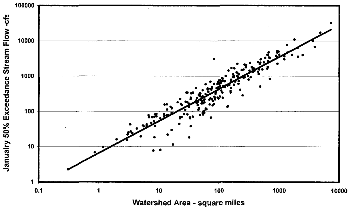
Figure 12. January 50-Percent Exceedance Stream Flow vs. Watershed Area for Gaged Streams West of the Cascade Crest Using Log-Transformed Data.
