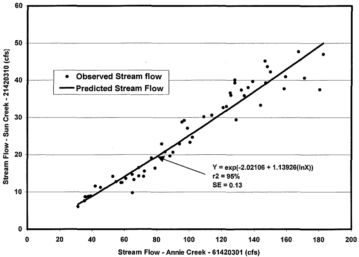
Figure 11. Relationship Between Stream Flow at Sun Creek (Gage 21420310 - Miscellaneous Measurements) and Annie Creek ( Gage 61420301– Mean Daily Flows).
