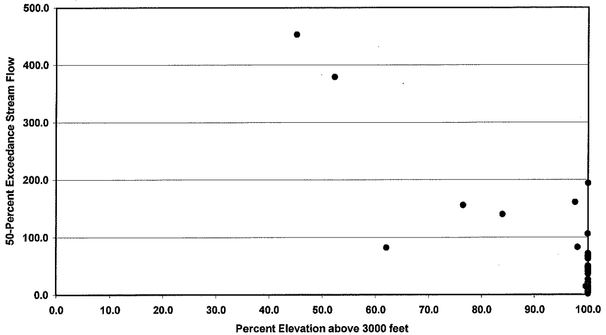
Figure 14. Percent Elevation above 3000 feet vs. 50-Percent Exceedance Stream Flow – for Gages East of Cascade Crest.
