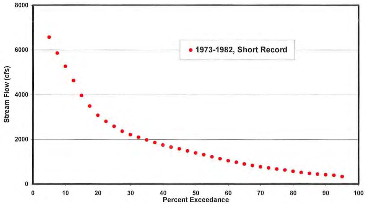
Figure 7. January Short Record Flow Duration Curve for the Wilson River near Tillamook, OR - Gage 14301500.
