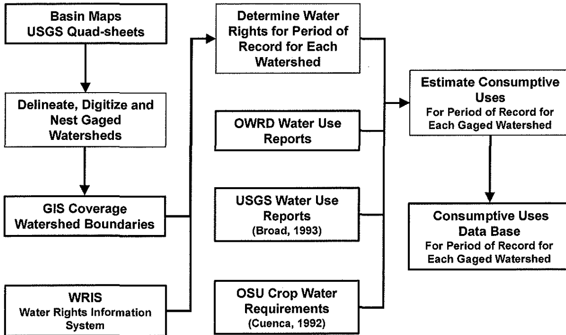
Figure 16. Storage and Consumptive Use Calculations – Correcting to Natural Stream Flow.
