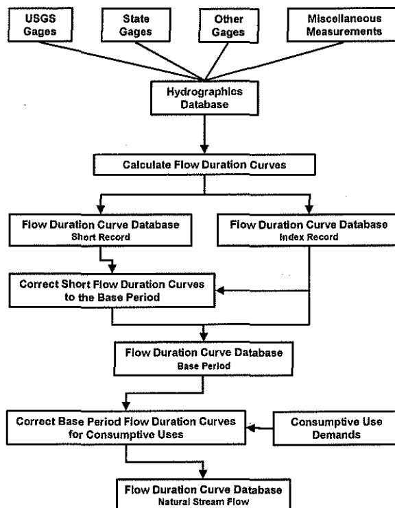
Figure 5. The Water Availability Methodology - Measured Watershed Stream Flow Analysis.
