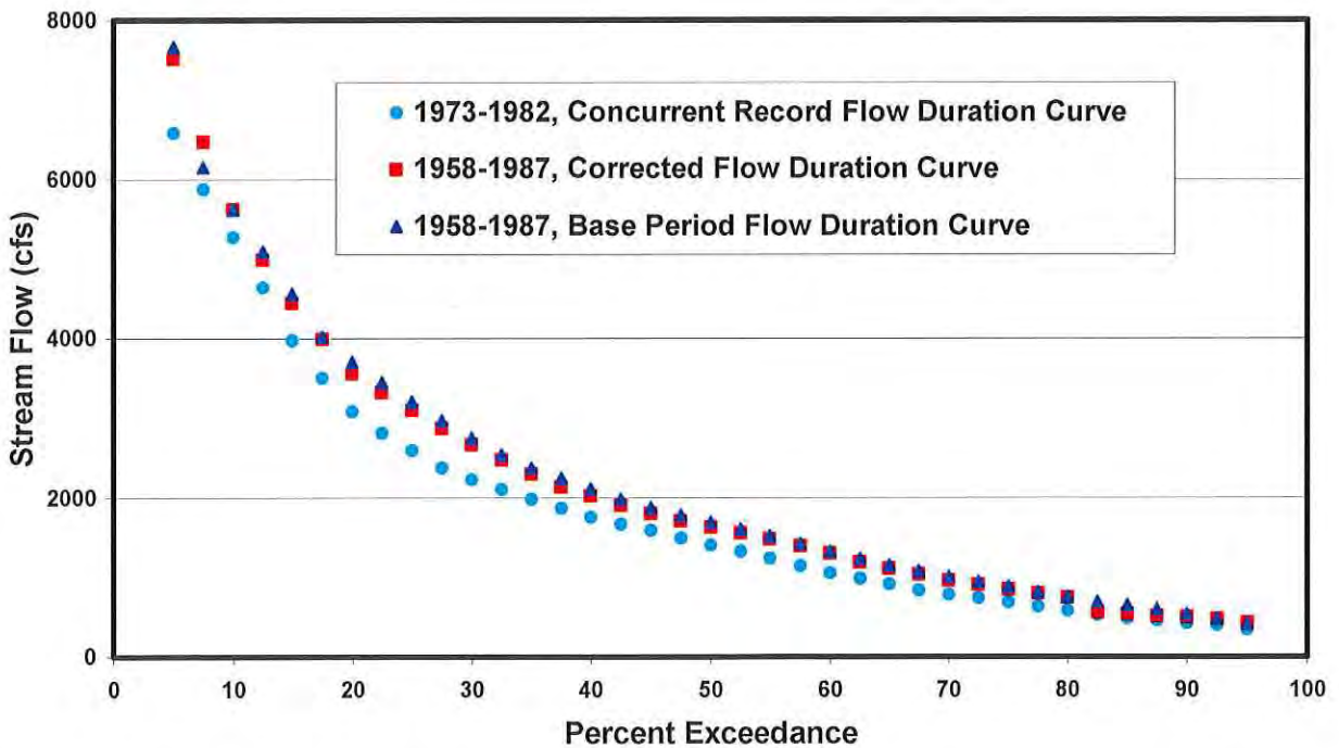
Figure 10. Comparison of January Flow Duration Curves for the Wilson River near Tillamook, OR – Gage 14301500.
