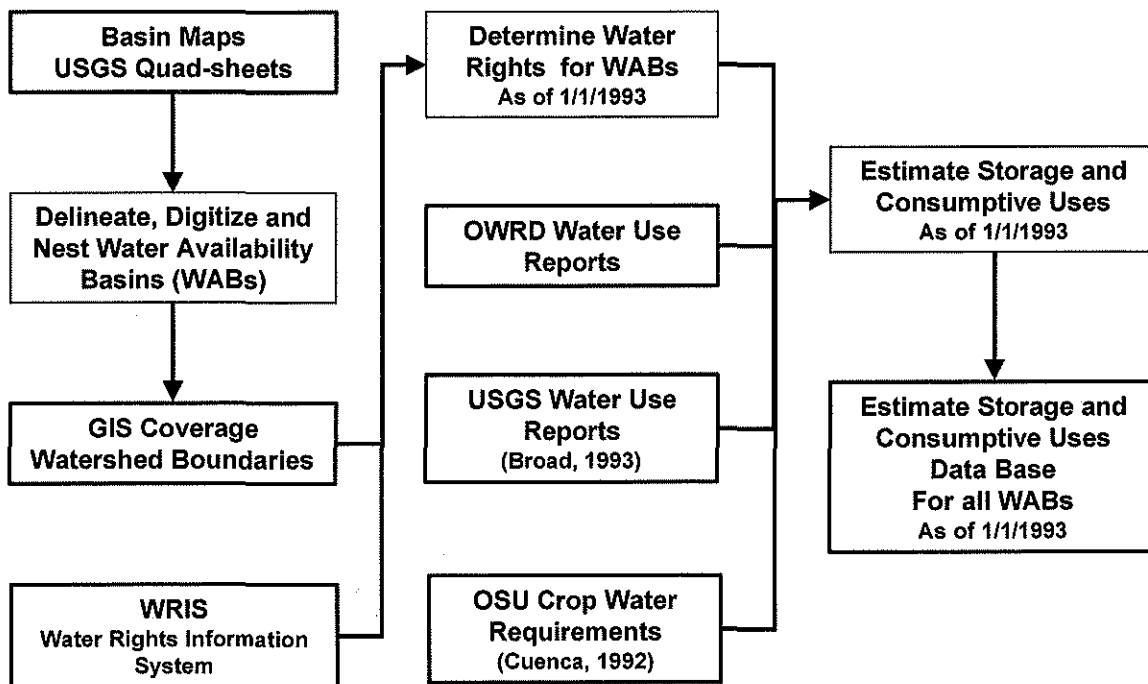
Figure 17. Storage and Consumptive Use Calculations – For the Water Availability Calculation.
