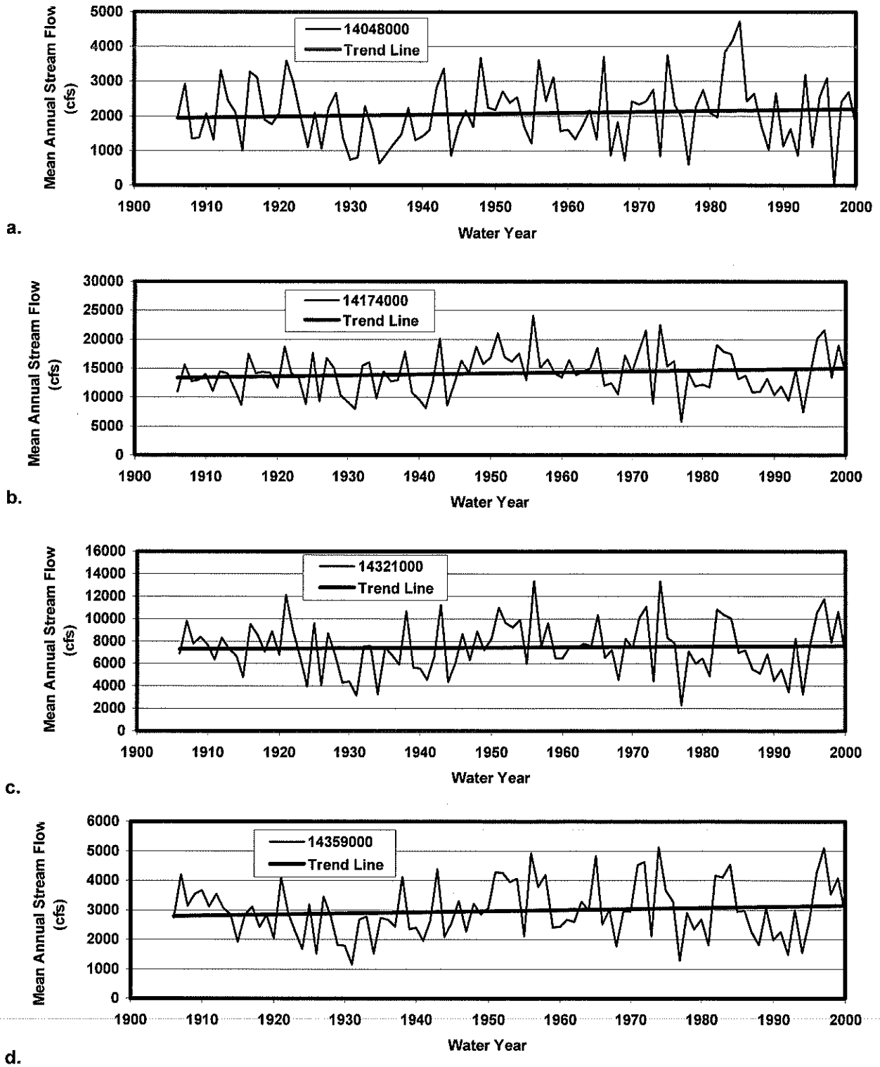
Figure 3. Mean Annual Stream Flow for Four Long-Term Gages in Oregon: a) 14048000, John Day River at McDonald Ferry, OR; b) 14174000, Willamette River at Albany, OR; c) 14321000, Umpqua River at Elkton, OR; and d) 14359000, Rogue River at Raygold near Central Point, OR. The trend lines were computed from a linear regression of the stream flows.
