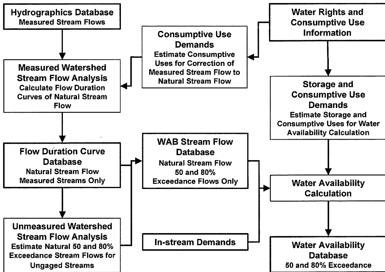
Figure 4. The Water Availability Methodology - an Overview.
