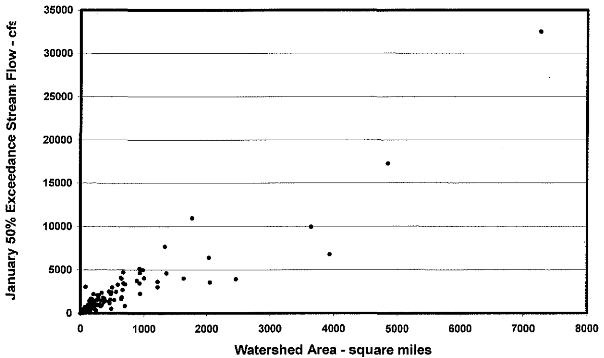
Figure 13. January 50-Percent Exceedance Stream Flow vs. Watershed Area for Gaged Streams West of the Cascade Crest Using Non-Log-Transformed Variables.
