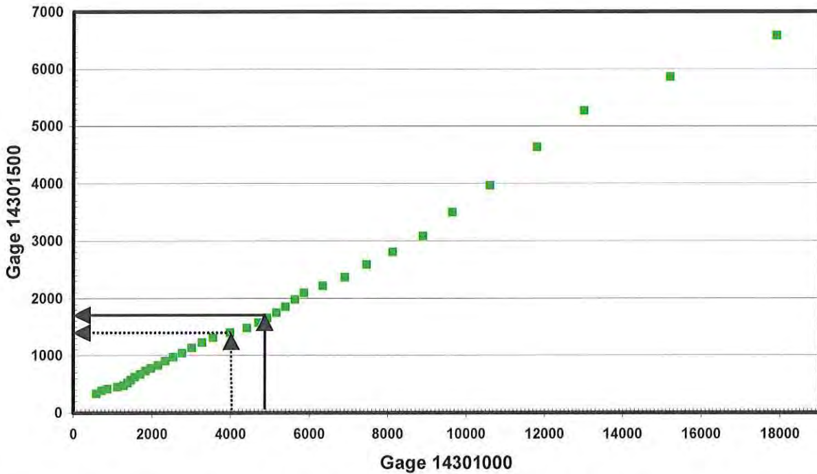
Figure 9. Relationship Between January Exceedance Stream Flows for the Nehalem River near Foss (Gage 14301000) and the Wilson River near Tillamook, OR (Gage 143015000) for the Concurrent Period 1973-1982.
