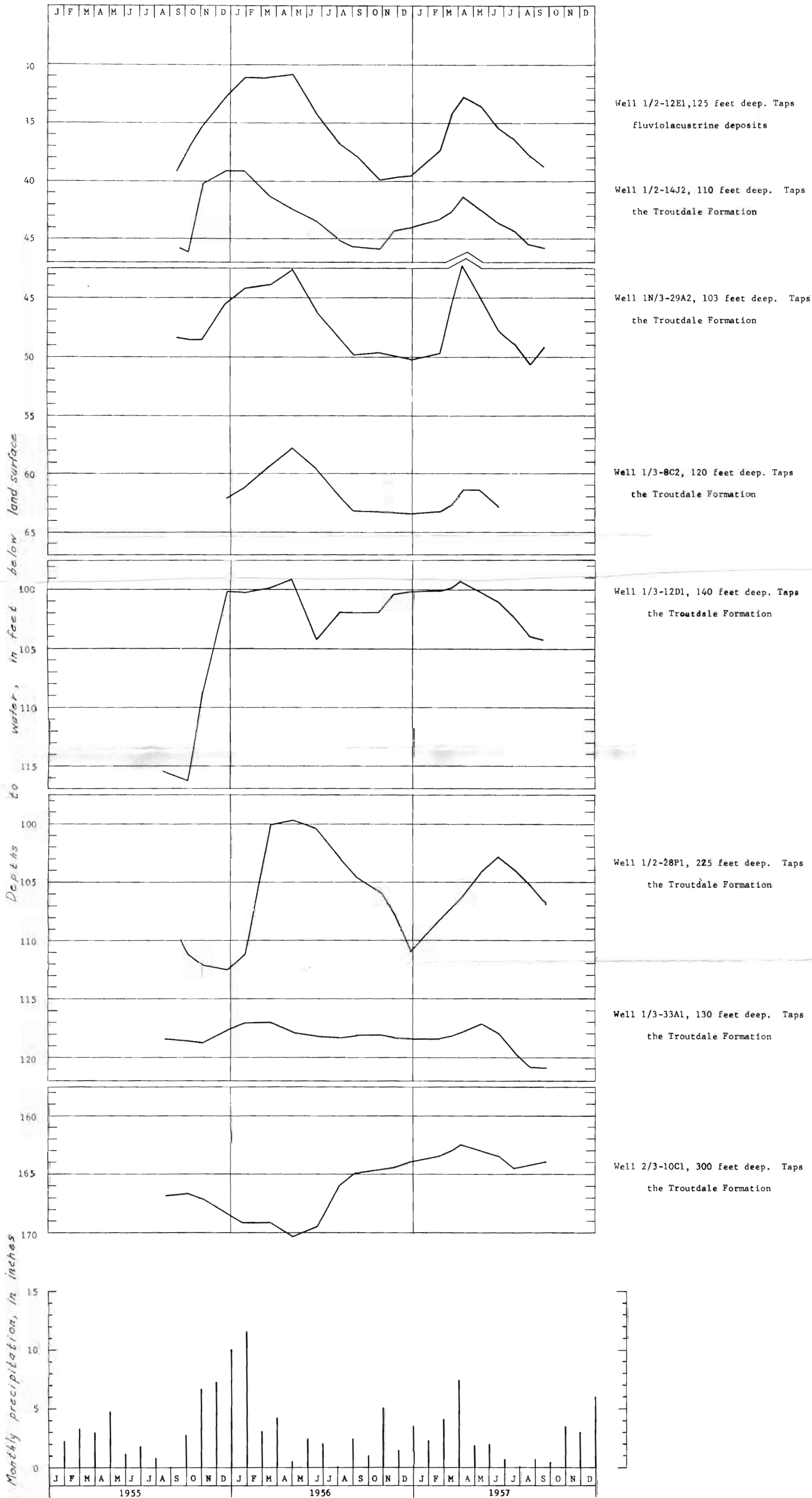
Figure 3.--Hydrographs of 8 wells in the East Portland area, Oregon, and monthly precipitation at Portland Airport for the period 1955-57.
