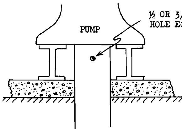
ACCESS PORT FOR MEASURING DEVICE
