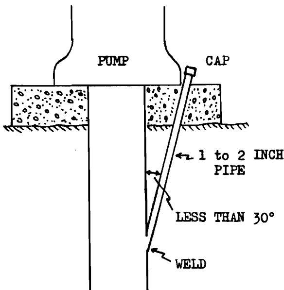
ACCESS PORT FOR MEASURING DEVICE
