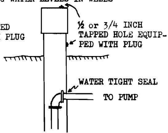
ACCESS PORT FOR MEASURING DEVICE
