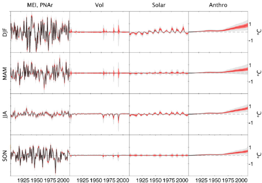
Figure 2: Drivers of air temperature in the Pacific Northwest during the 20 th century. Taken from Abatzoglou et al., 2014.
