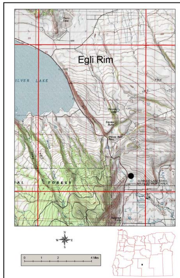
Figure 1. Location map. Showing location of the Egli Rim 7.5-minute quadrangle (outlined in red). The black dot is the location of drilling the thermal gradient well ARRA SL-1
