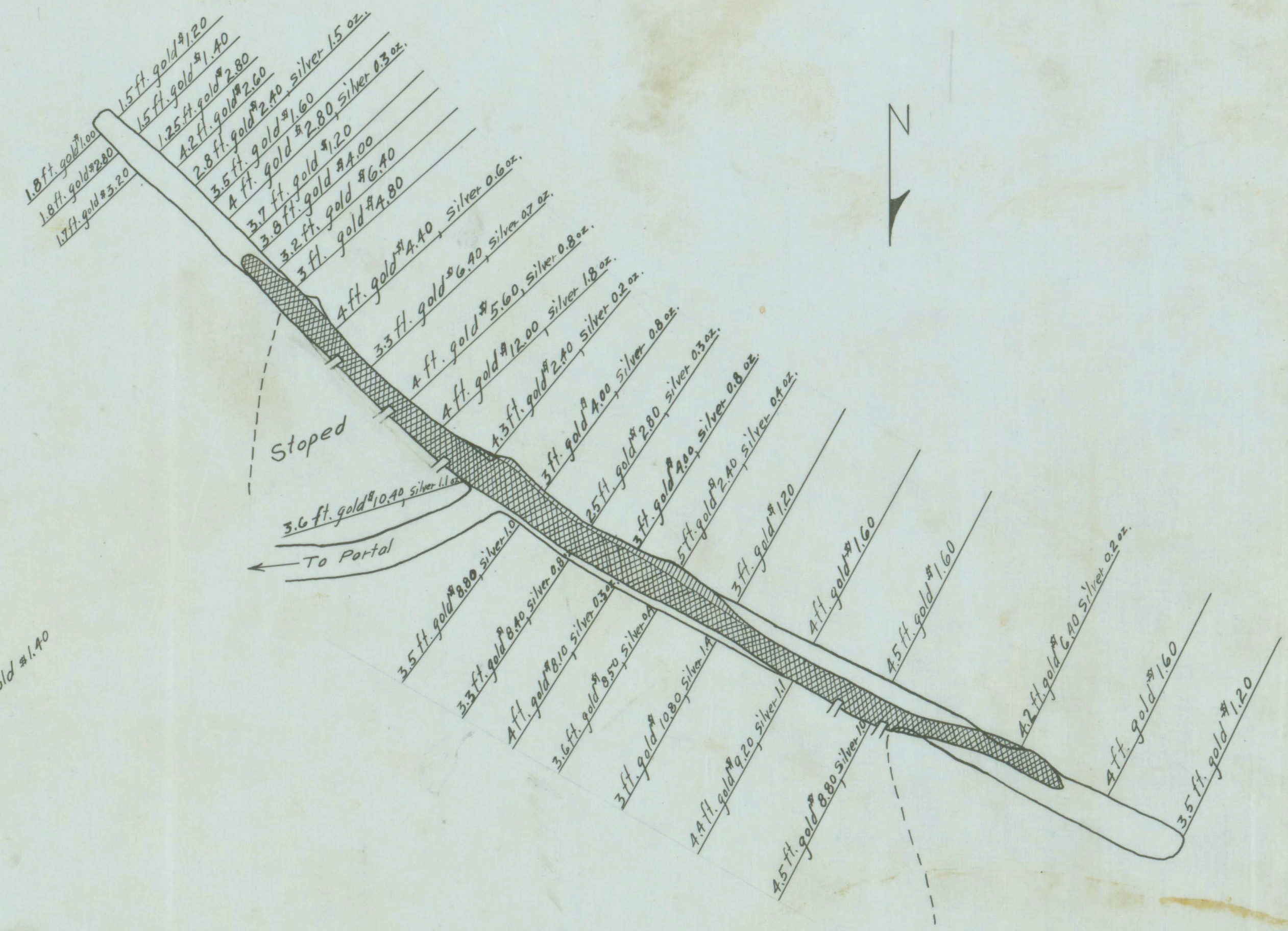
No. 1 ORE SHOOT scale - 1 in. = 20 ft.
