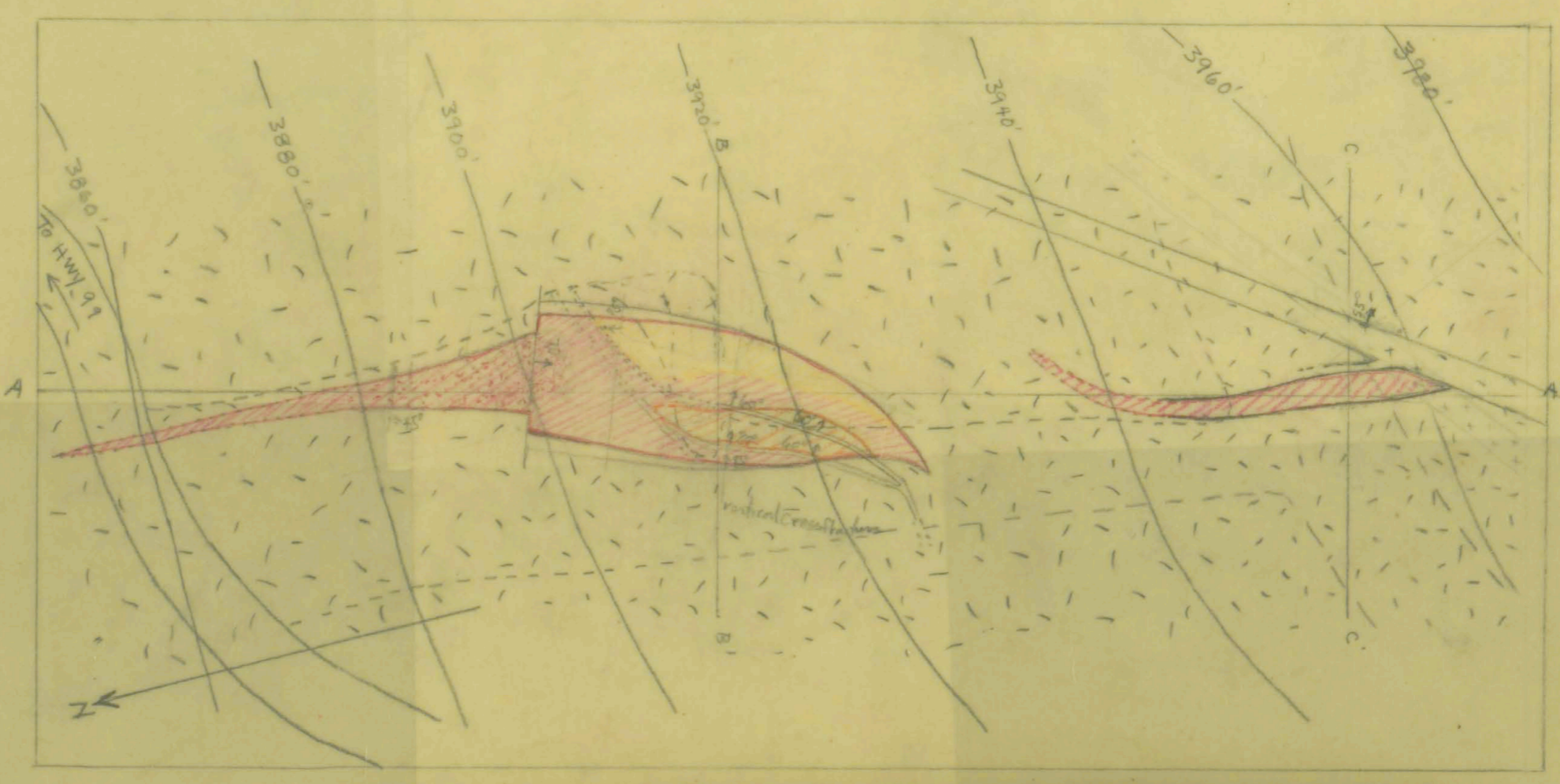
SECTION A-A' BRATCHER MINE
