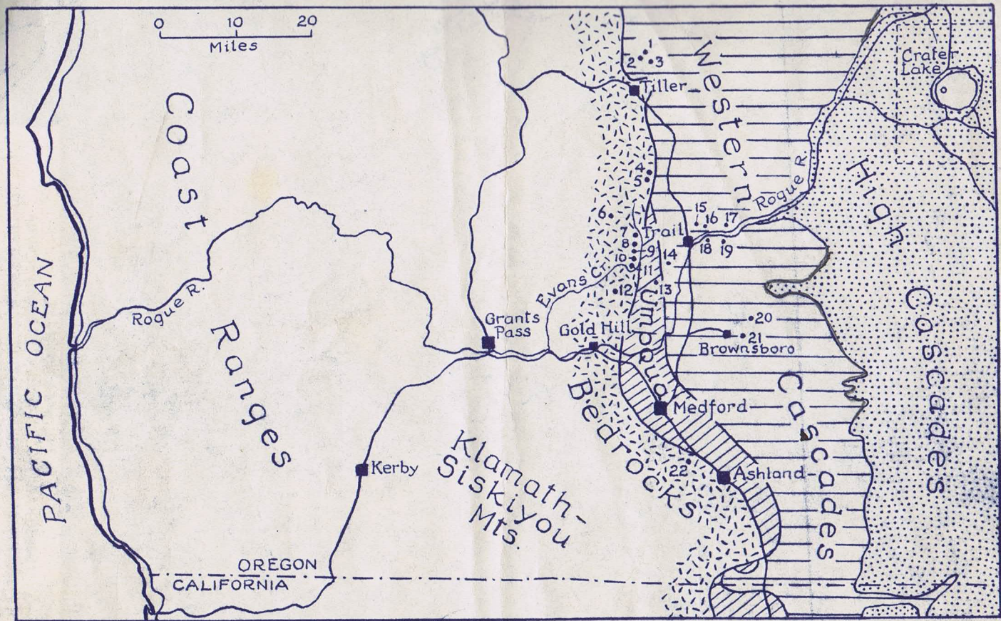
Figure . Sketch-map of Southwest Oregon showing the location of the main quicksilver deposits referred to in the text. 1- Buena Vista ; 2- Maud S. ; 3- James R. ; 4- Nivison and Thomason ; 5- Red Cloud ; 6- Bonita ; 7- Roxana ; 8- War Eagle ; 9- Palomar ; 10- Dave Force ; 11- Chisholm ; 12- Mountain King ; 13- Cinnabar Mt. ; 14- Sagar and Hull ; 15- Pitt View ; 16- Poole and Pence ; 17- Rayome and Midnight ; 18- Ash ; 19- Red Chief ; 20- Call of the Wild ; 21- Stanley and Brown ; 22- Phillips. Deposits 6 to 14 inclusive belong to the Meadows district ; a few of the principal highways are indicated.
