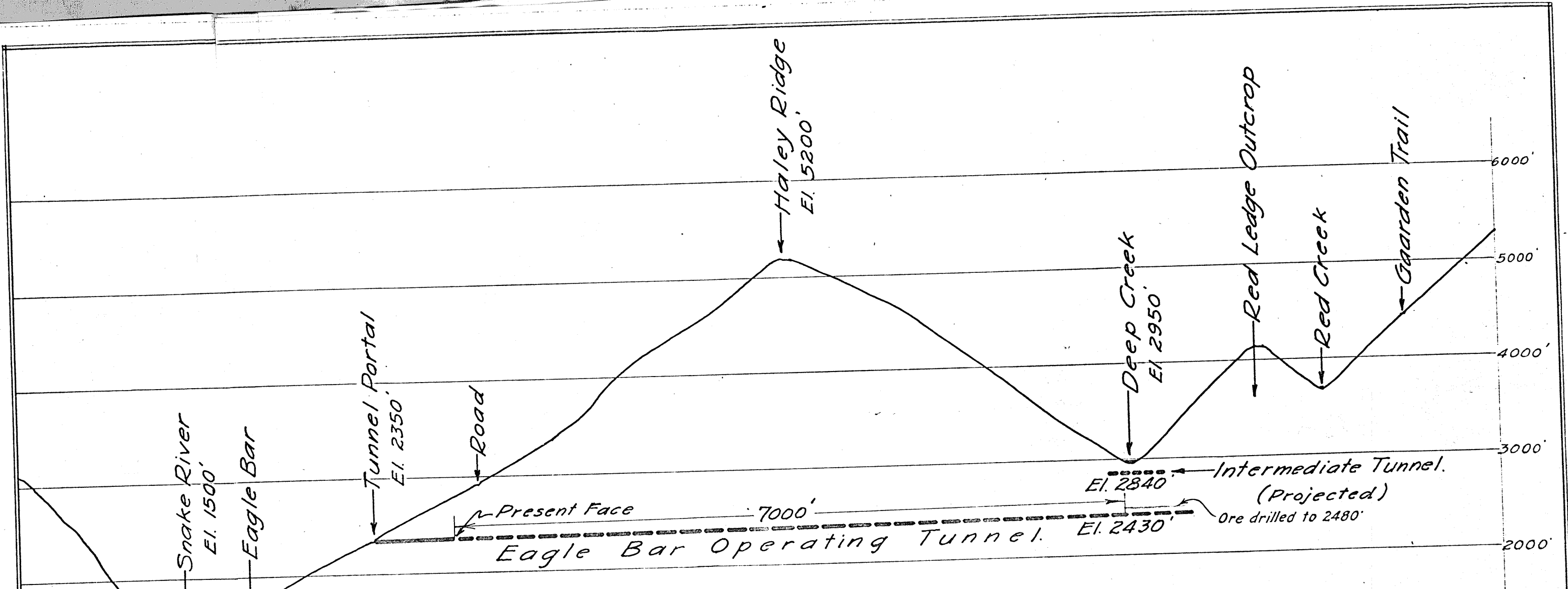
CROSS SECTION OF HALEY RIDGE ALONG THE PROPOSED OPERATING TUNNEL FROM EAGLE BAR TO DEEP CREEK.
