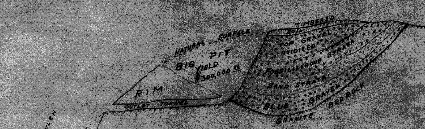
VERTICAL SECTION THRU OLD CARSON PIT SHOWING THE STRATIFICATION OF DEPOSIT. SCALE ONE INCH = 200 FT.
