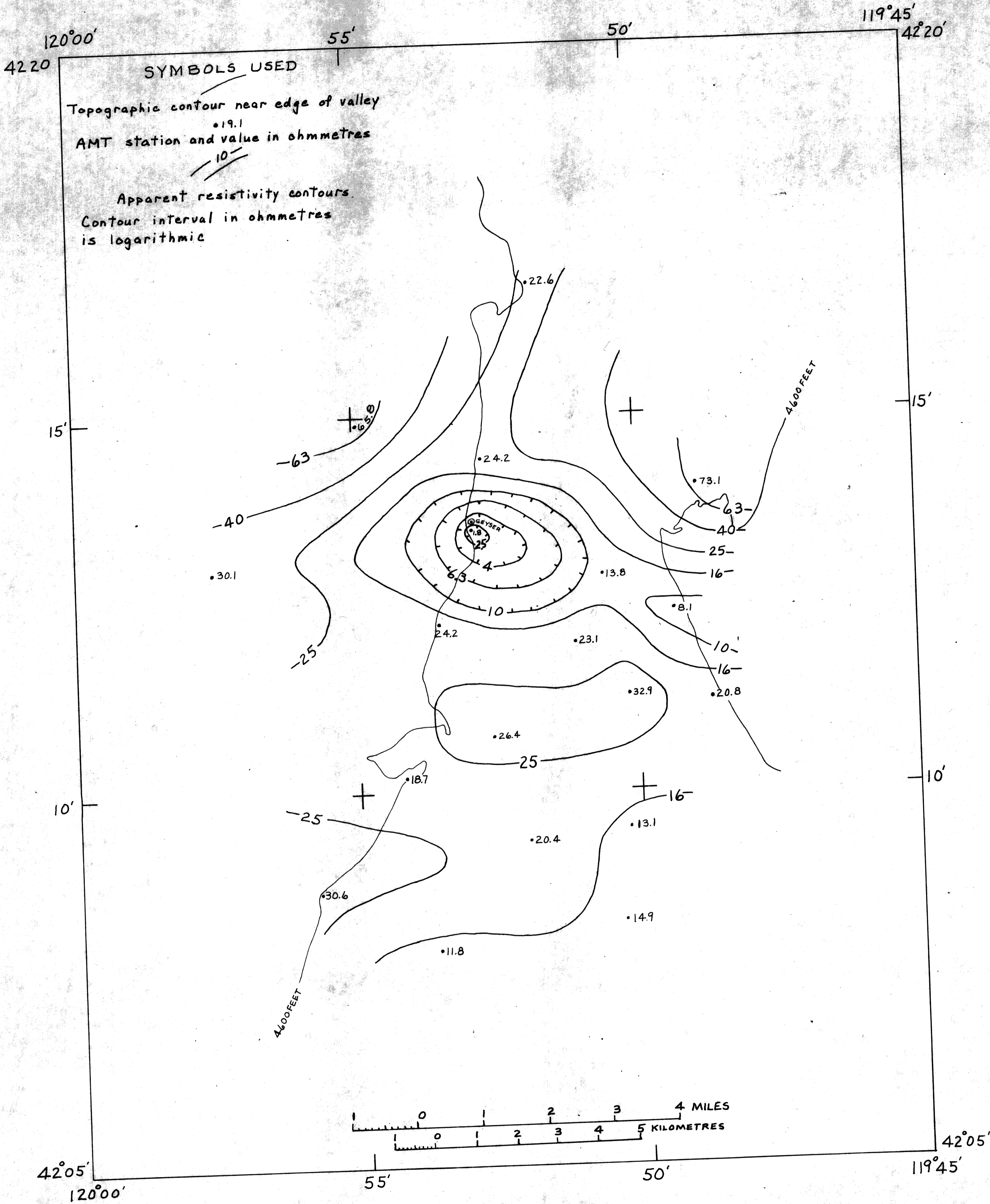
AUDIO-MAGNETOTELLURIC APPARENT RESISTIVITY MAPS SOUTHERN WARNER VALLEY, LAKE COUNTY, OREGON 27 HERTZ; TELLURIC LINE NORTH-SOUTH BY
