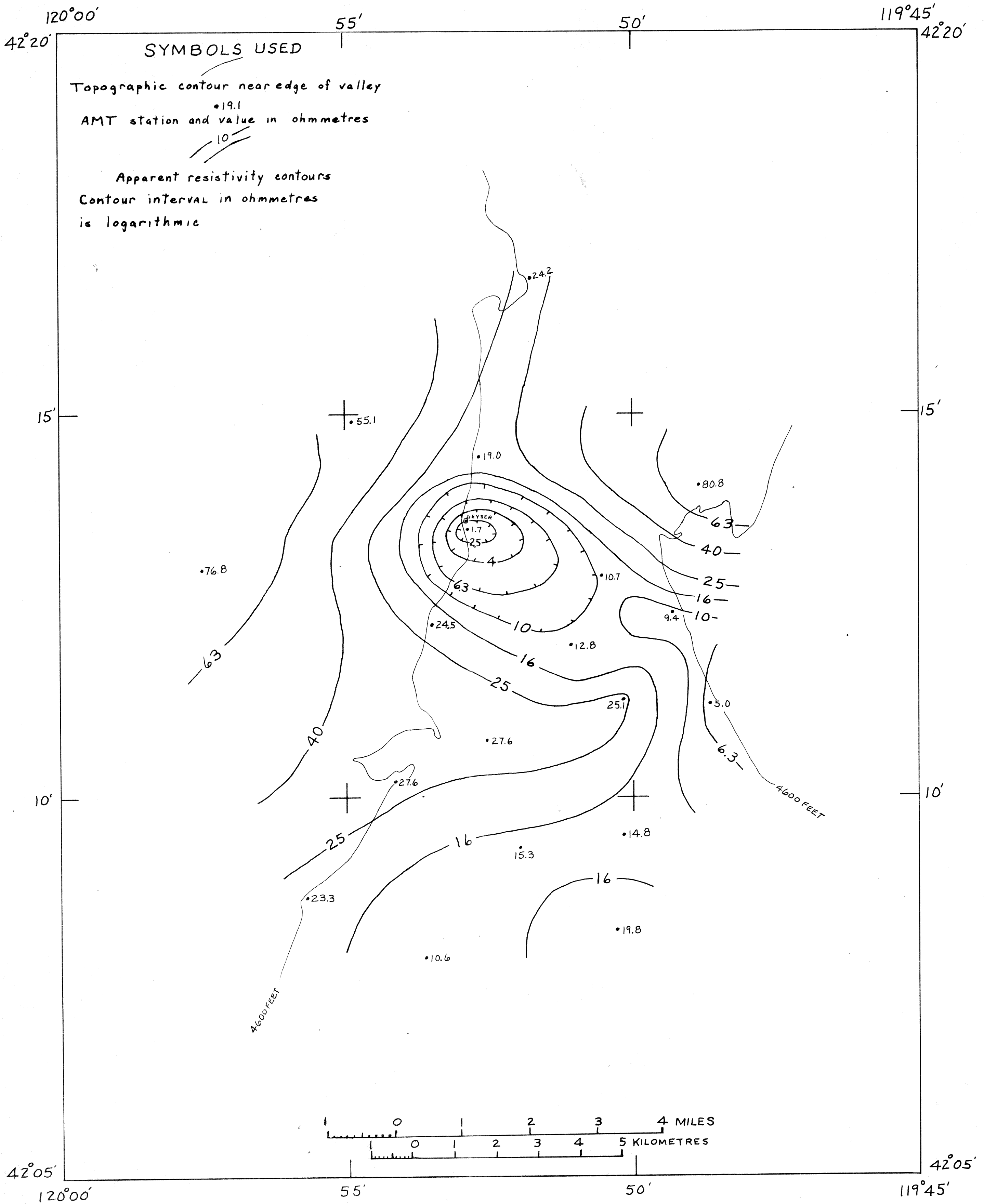
AUDIO-MAGNETOTELLURIC APPARENT RESISTIVITY MAPS SOUTHERN WARNER VALLEY, LAKE COUNTY, OREGON 27 HERTZ; TELLURIC LINE EAST-WEST BY
