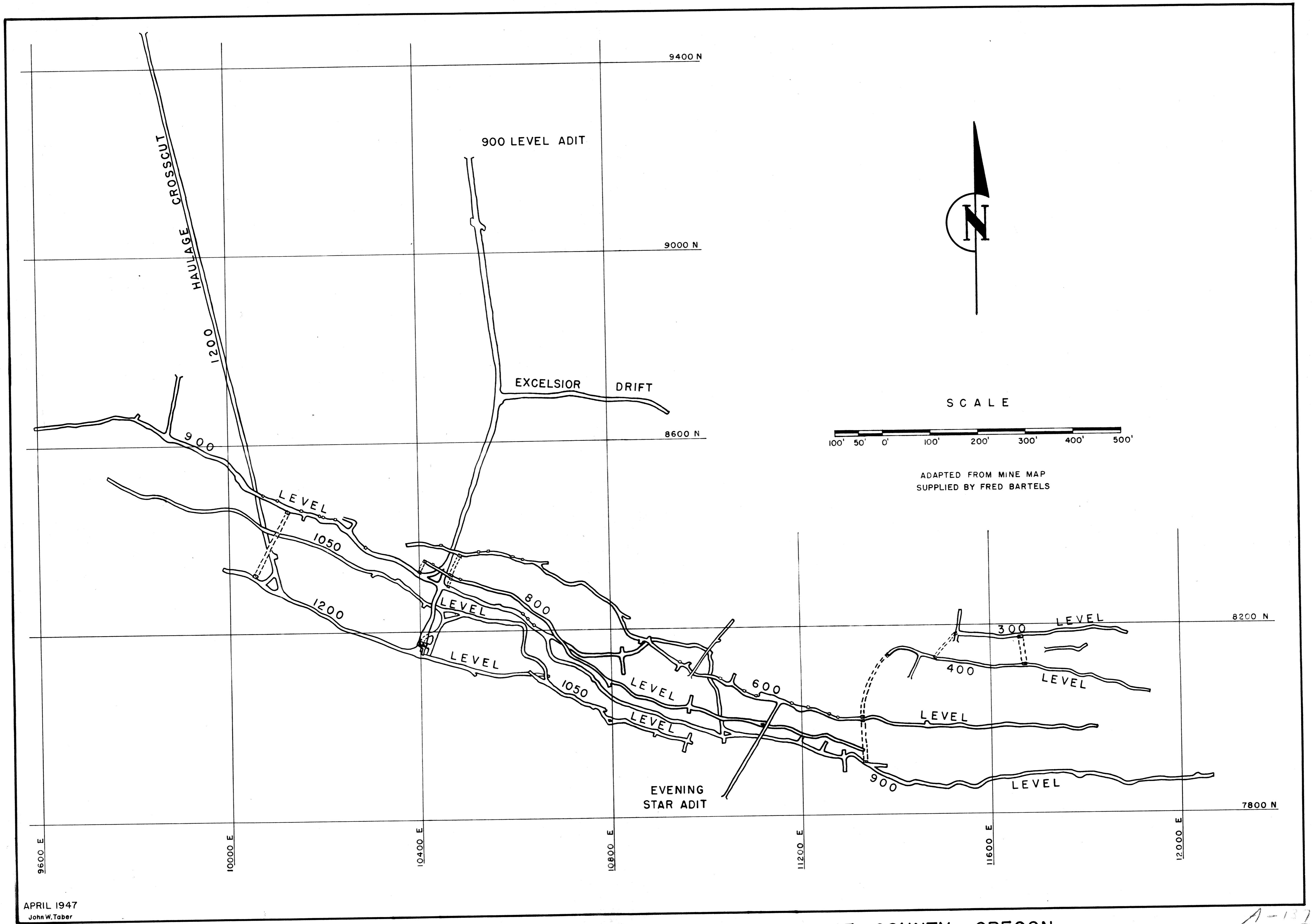
FIG. 3 COMPOSITE PLAN OF CHAMPION MINE, LANE COUNTY, OREGON
