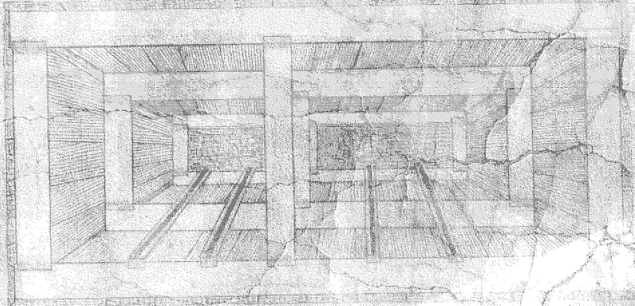
Showing the Double End of the Working Tunnel as a whole. Scale 2 1/2 to an inch.
