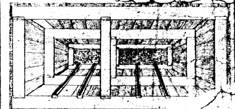
DIAGRAM Showing the Double Working Incline as constructed. Scale 2 1/2 to an Inch
