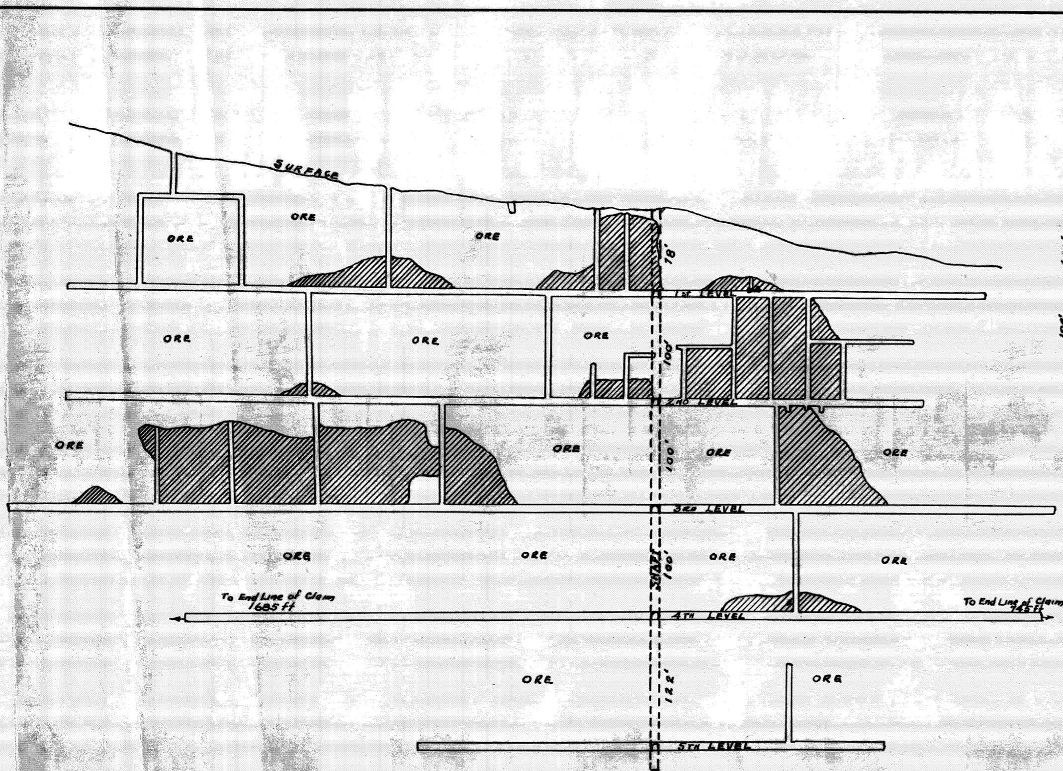
SECTION OF HUMBOLDT MINE SHOWING DEVELOPMENT - ORE MINED
