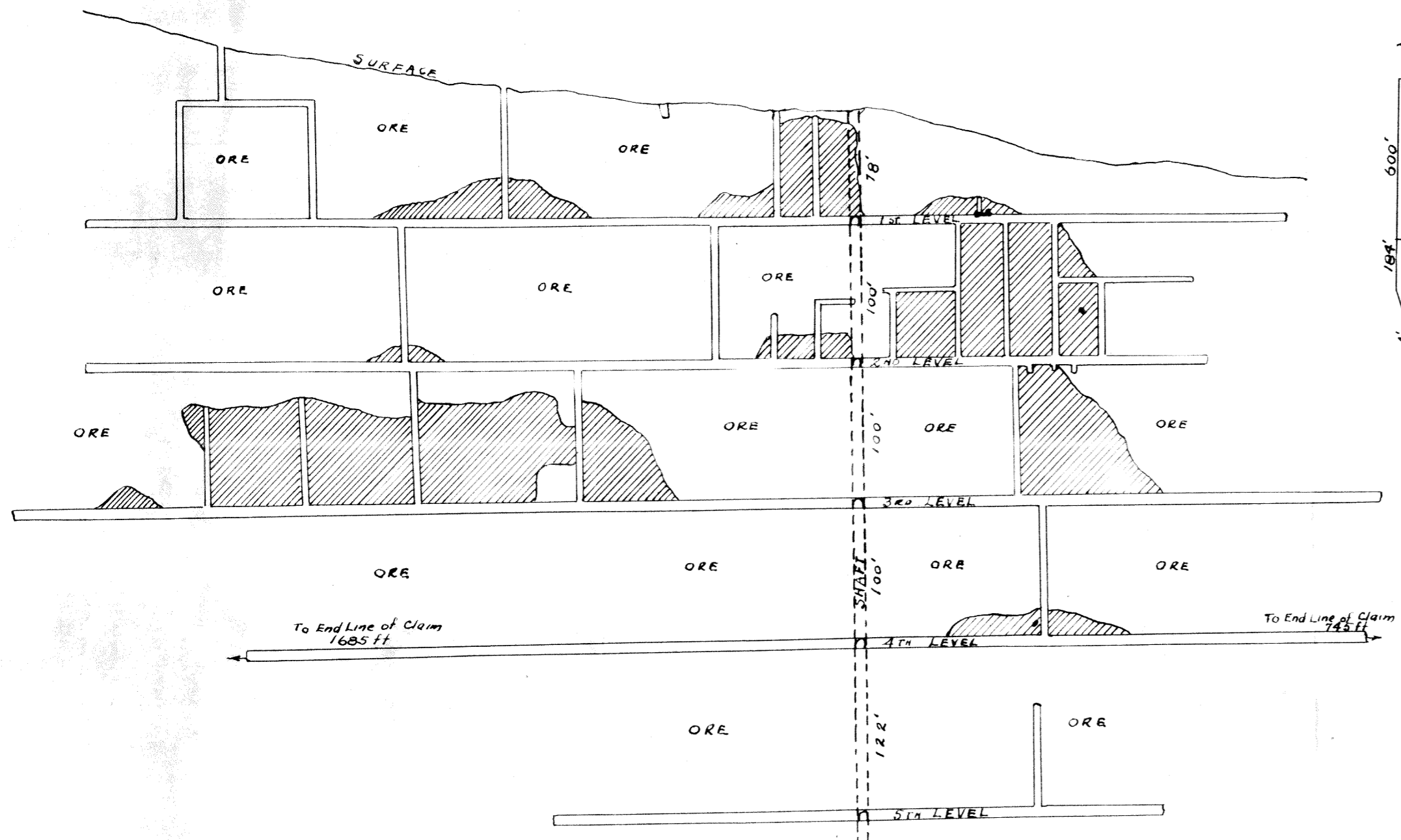
SECTION OF HUMBOLDT MINE SHOWING DEVELOPMENT - ORE MINED
