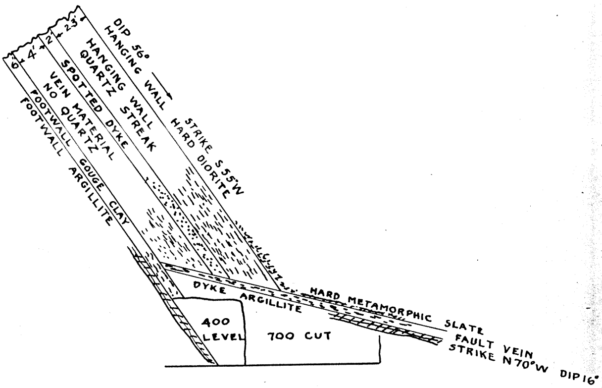
SKETCH CROSS SECTION ON LINE A-A AS SHOWN ON PLATE 2 SHOWING INTERSECTION OF VEINS ON FAULT PLANE LOOKING SOUTH 55° WEST
