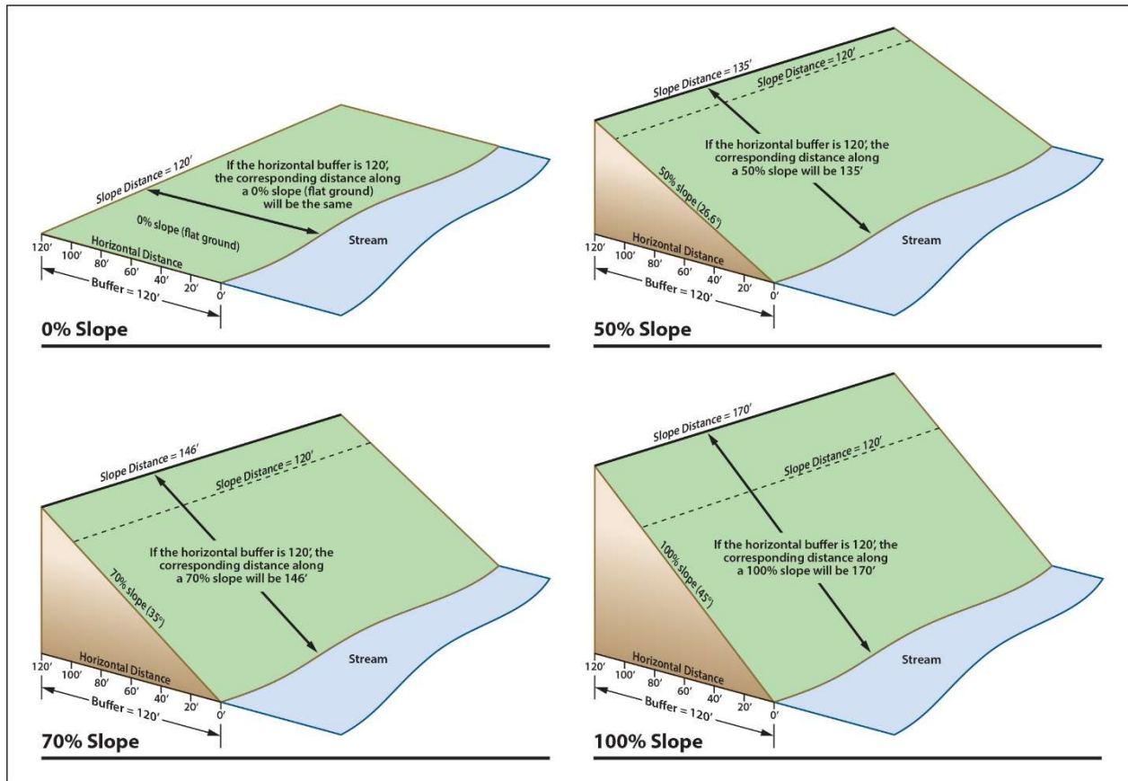
Examples of the Horizontal Distance Measurement of a 120-foot Riparian Conservation Area
