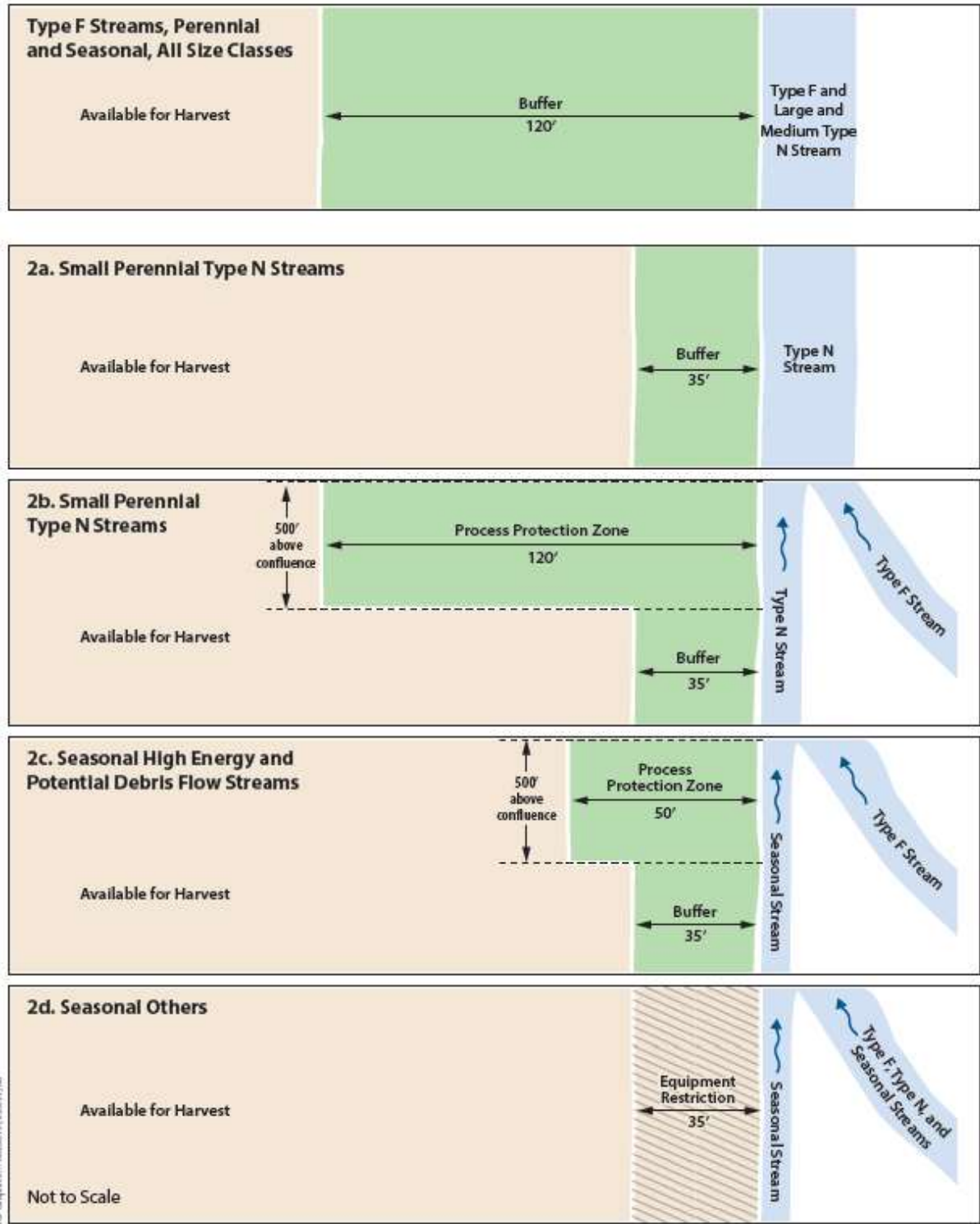
Riparian Conservation Areas on Type F and N Streams, Perennial and Seasonal, All Size Classes
