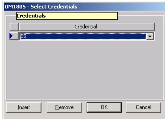
Figure 5: “Credentials” Pop-up
