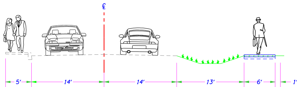
PROPOSED "B" STREET (TERREBONNE)
