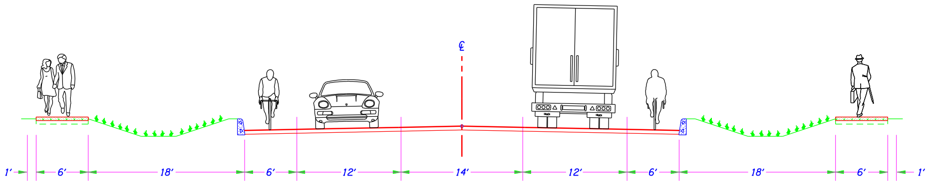
PROPOSED HIGHWAY 97 CROSS-SECTION (TERREBONNE)
