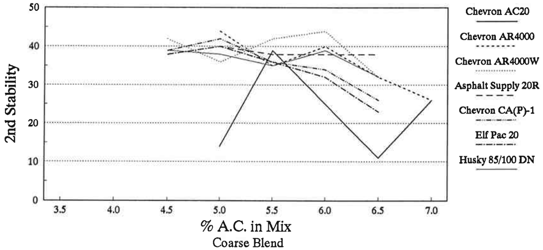
FIGURE 4B: Individual Stability Test Results 2nd Compaction
